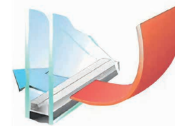
aluminium spacer
